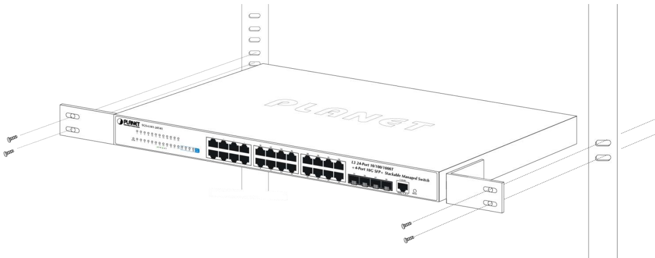
Figure 2-2-2-2 Mounting SGS-6350 Series in a Rack
