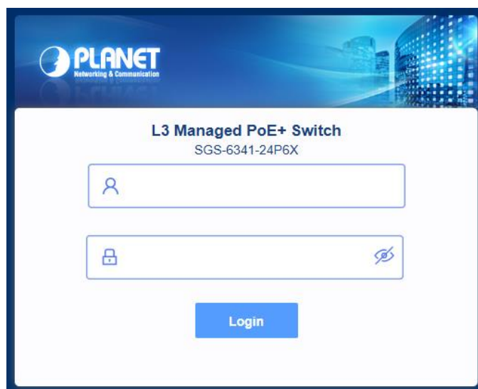
Figure 3-9-1 Login Screen
