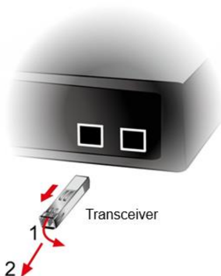
Figure 2-2.3: How to Pull Out the Transceiver
